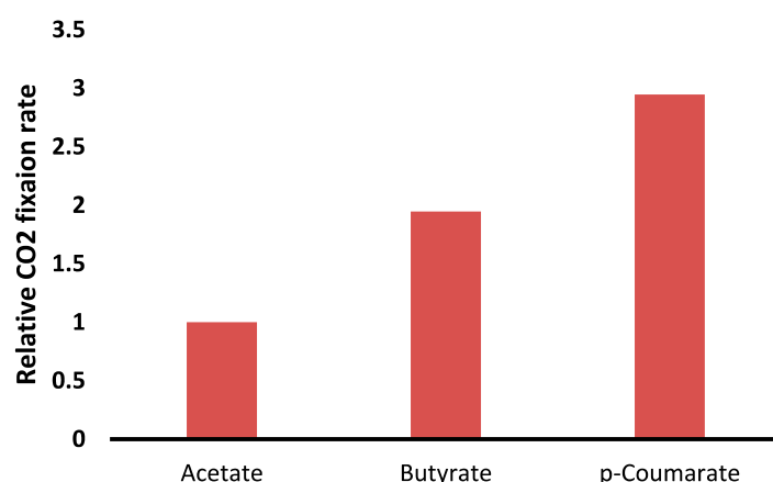
Fig. 8: Relative predicted rate of CO 2 fixation during growth on acetate, butyrate, and p -coumarate.
