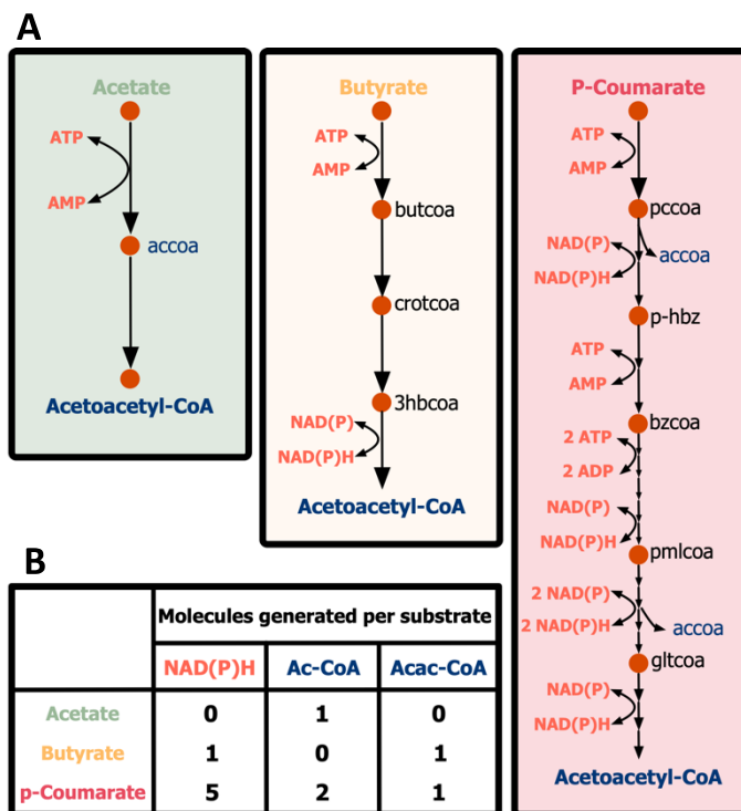
Fig. 5: Substrate consumption of the three modeled carbon sources: acetate, butyrate, and p -coumarate depicting the (A) breakdown pathways and the (B) relevant cofactors and PHB precursors produced from each carbon source.
