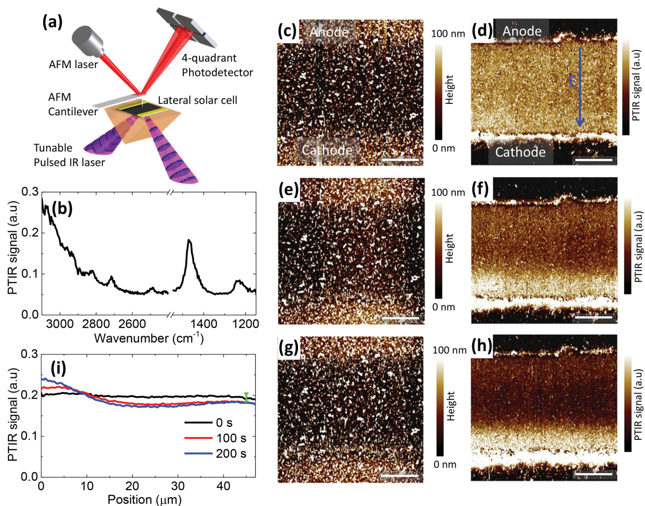
Figure 2. a) Schematic illustration of the PTIR measurement. b) A representative absorption spectrum obtained at the center of the device. c,e,g) Topography maps (80 μm × 80 μm) of the MAPbI 3 film of the same sample area before (c), after 100 s (e) and after 200 s (g) electrical poling, respectively. The poling field was 1.6 V μm -1 . d,f,h) Corresponding PTIR images for the CH 3 asymmetric deformation absorption of the methylammonium ion (1468 cm -1 ) obtained before (d), after 100 s (f) and after 200 s (h) electrical poling, respectively. i) Line-averaged profile (perovskite region only) of 256 vertical lines in the PTIR images before and after electrical poling, showing the redistribution of the MA + ions. The error bar represents the uncertainty of the background level when comparing data from different scans. All scale bars are 20 μm.
