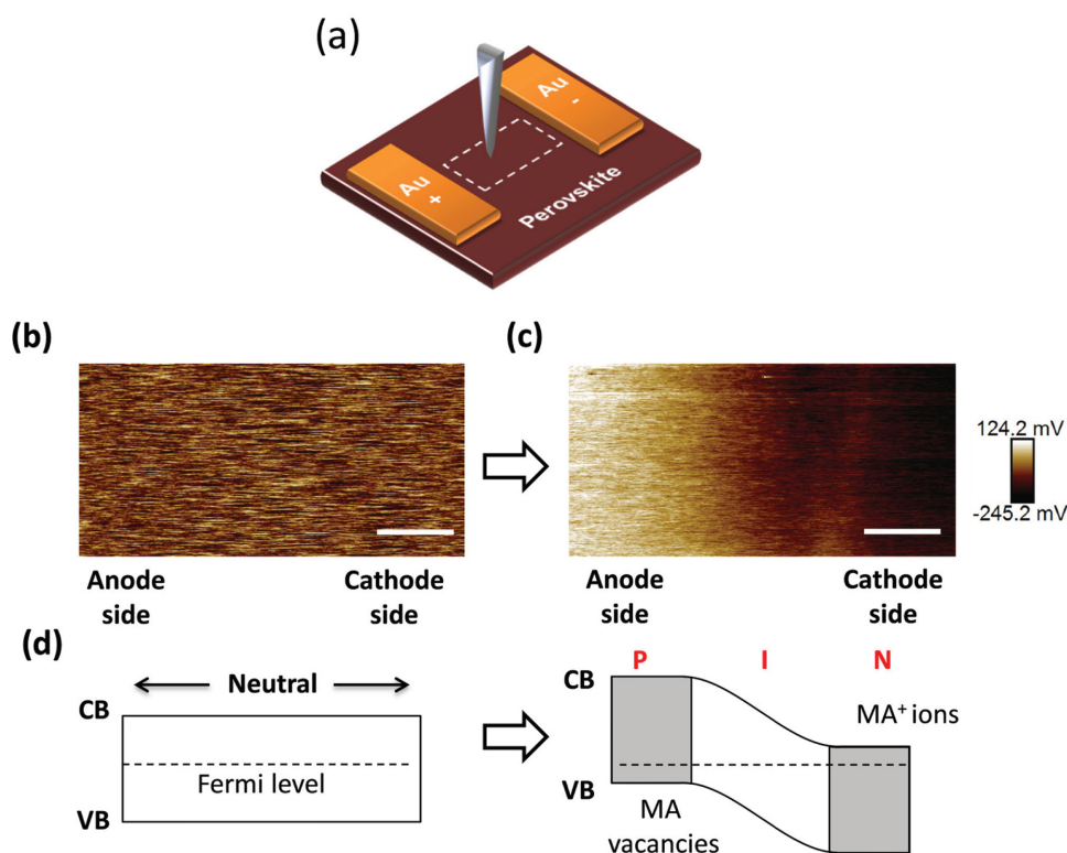
Figure 3. a) Schematic of the KPFM measurements of the lateral structure devices, where the white dash line indicates the location of the scanning region. b,c) KPFM potential images of the MAPbI 3 thin films between the two Au electrodes before (b) and after (c) electrical poling (1.2 V \mu\text{m}^{-1} for 100 s), respectively. The electrode spacing is 50 \mu\text{m} . The scale bar is 6 \mu\text{m} ; d) energy diagram of the MAPbI 3 film before and after electrical poling, where p-i-n junction was formed due to the accumulation of MA + ions (vacancies) in proximity of the cathode (anode) side.
