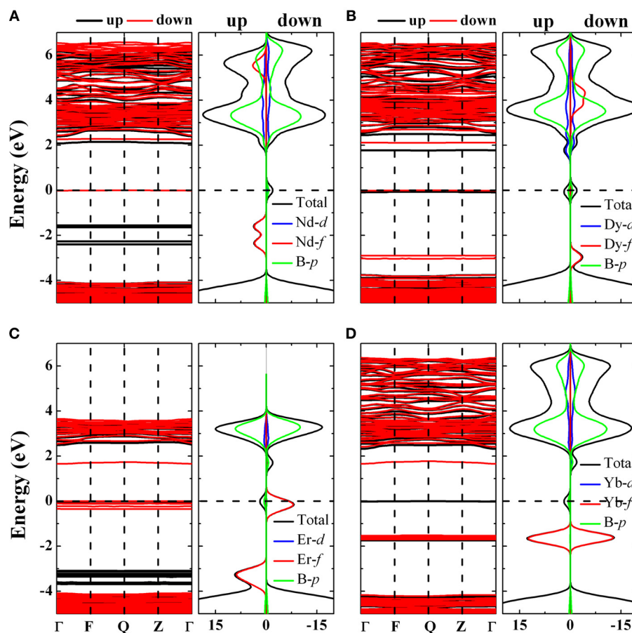
FIGURE 10 | The band structure and density of states of \text{Li}_{15}\text{B}_{32}\text{O}_{56}\text{Nd} (A), \text{Li}_{15}\text{B}_{32}\text{O}_{56}\text{Dy} (B), \text{Li}_{15}\text{B}_{32}\text{O}_{56}\text{Er} (C), \text{Li}_{15}\text{B}_{32}\text{O}_{56}\text{Yb} (D). In band structure plots vs. wave vector, spin up is black and spin down is red, while in the
