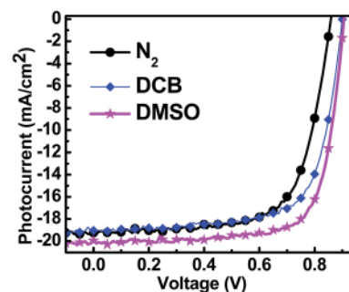
Fig. 4 Photocurrent ( J ) versus voltage ( V ) curves for solar cells fabricated under atmosphere of N_2 and DCB, and DMSO vapors, respectively.
