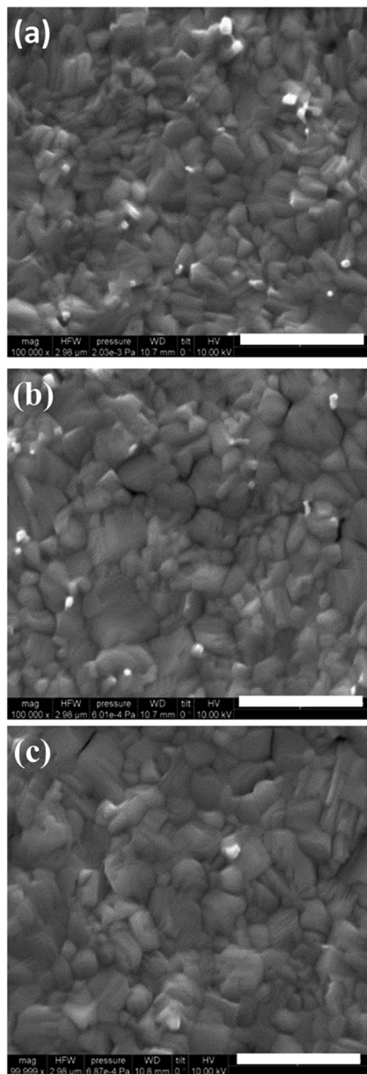
Fig. 2 The surface topography measured by SEM for different perovskite films fabricated in the atmosphere of (a) N_2 , (b) DCB vapor, and (c) DMSO vapor, respectively. The scale bar is 1 \mu m .
