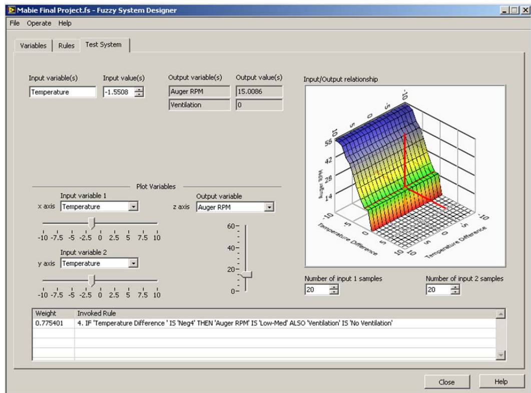
Figure A.8. Fuzzy System Test.
