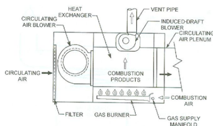
Fig. 4 Horizontal Category I Furnace with Induced-Draft Blower
