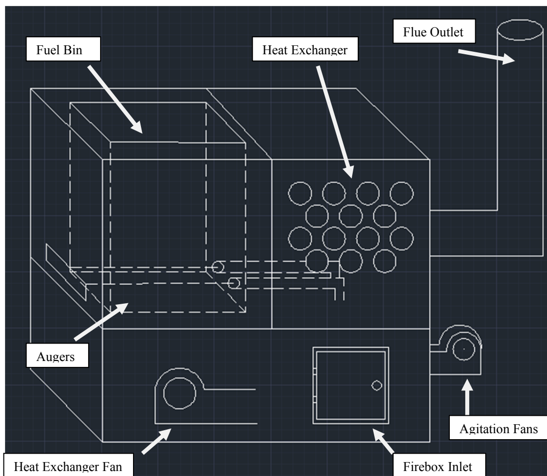
Figure 2.3. Biomass Furnace Side View Schematic.
