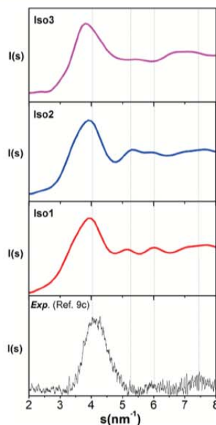
Figure 4. Comparison of the experimental XRD curve with simulated XRD curves of Iso1–Iso3 .
