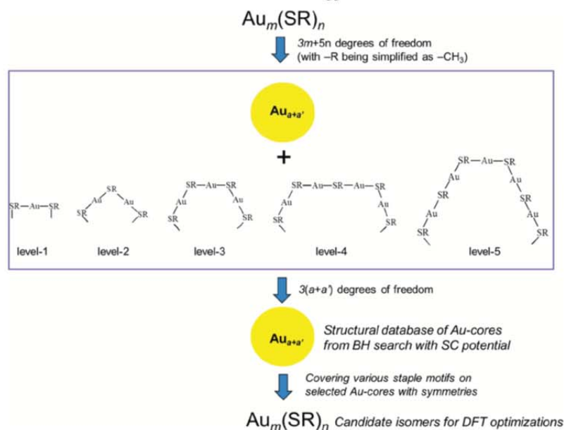
Scheme 2. Illustration of the Force-Field Based Divide-and-Protect Approach
