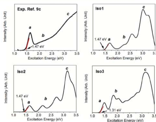
Figure 2. Comparison of the experimental (upper left panel) and theoretical UV–vis absorption spectra of \text{Au}_{24}(\text{SR})_{20} . In theoretical calculations, the –R group is simplified as –CH 3 . The red lines define the optical band edge. The experimental curve is taken from ref 9c.
