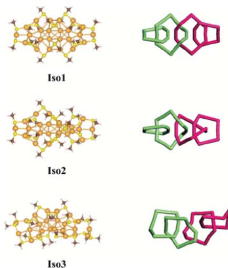
Figure 1. Optimized structures of three lowest-lying isomers Iso1–Iso3 (left panel). The methyl groups are removed for clarity in the topological structural model (right panel). The Au, S, C, and H atoms are in khaki, yellow, gray, and white colors, respectively (left panel). Another atomic view of interlocked topological structural model is given in the Supporting Information with detailed Cartesian coordinates (the final section of SI).
