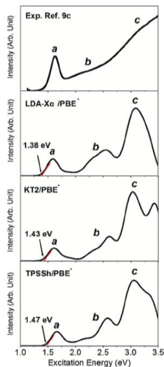
Figure 3. Comparison of the experimental and theoretical UV-vis absorption spectra of Iso1 based on different geometries. *The geometric structure of Iso1 is reoptimized based on LDA-X/TZP, KT2/TZP and TPSSH/LANL2DZ + 6-31G(d) level of theory, respectively; the excitation energy is computed using PBE functional. The red lines define the optical band edge. The experimental curve is taken from ref 9c.
