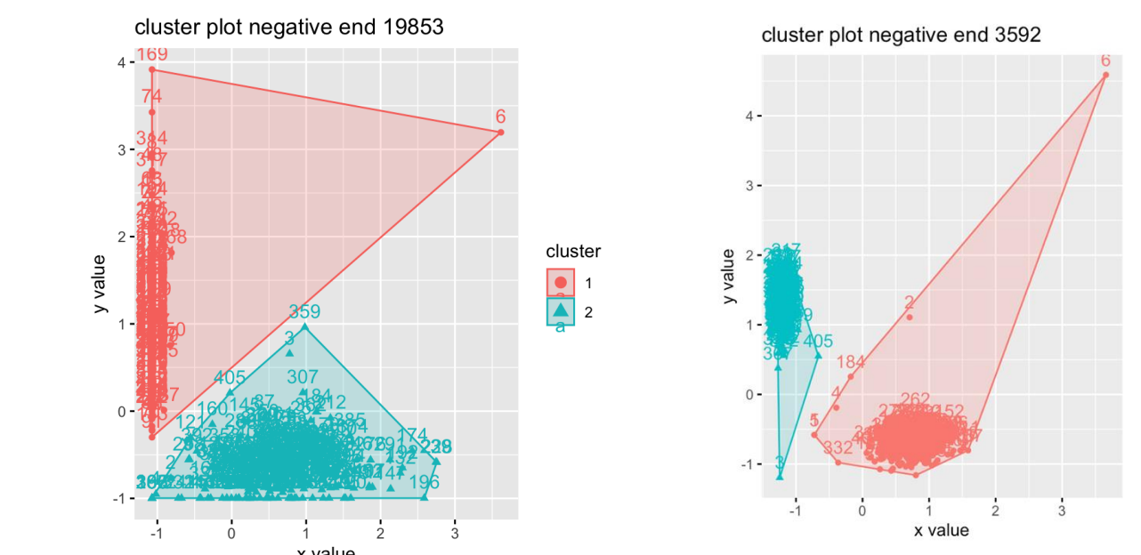
Figure 2. Two example of clusters that are a GSS AltT or AltD events from rice population;
