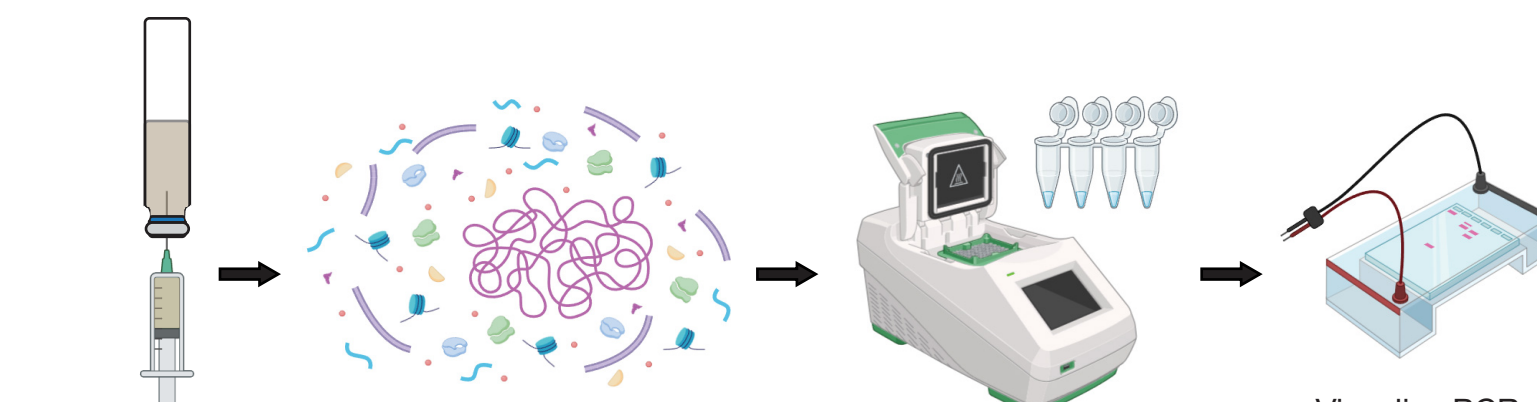
Figure 12: Method of diagnostic PCR to screen transformants for integration of terpene gene into the methanogen genome.
