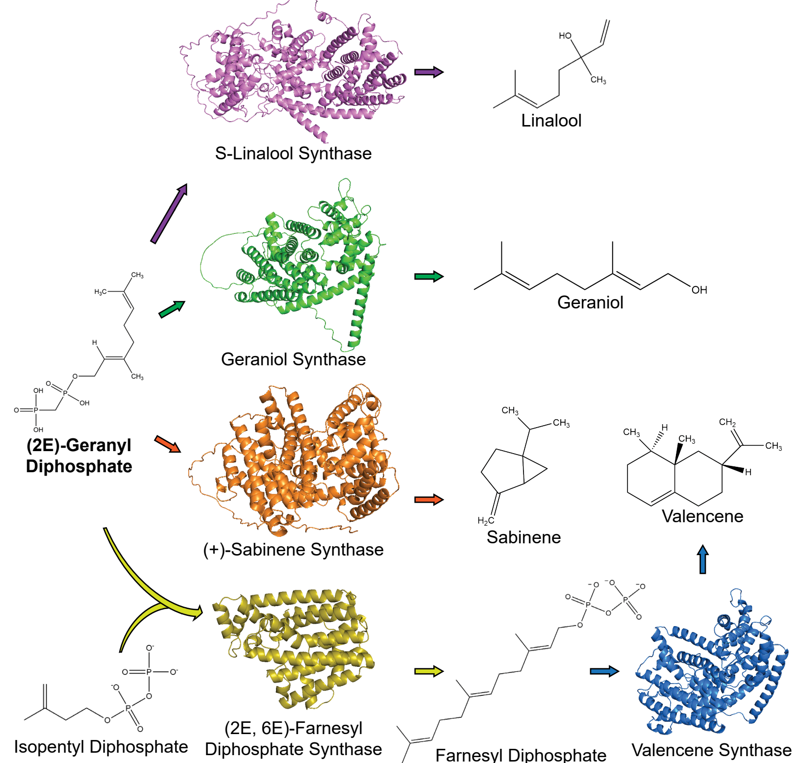
Figure 1: Biochemical pathway of terpenes and their enzymes. Enzyme structures are predicted by AlphaFold and visualized on Pymol. UniProt: Q96376, Q6USK1, O81193, A0A7J9PTF8, Q6Q3H2.
