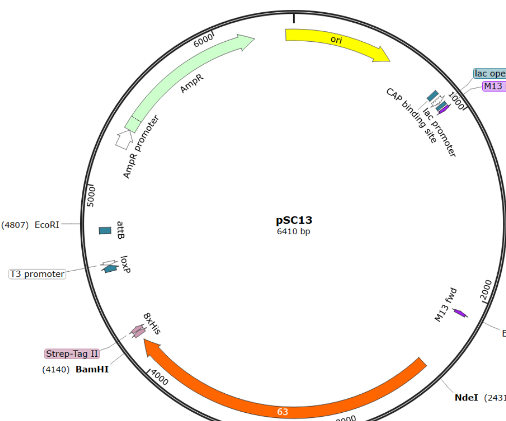
Figure 3: Map of pSC13. Backbone is pNB730 digested with NdeI and BamHI, and the insert is a terpene gene optimized for M. acetivorans .
