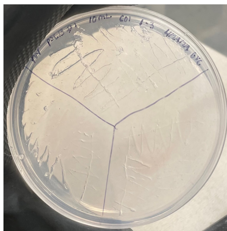
Figure 8: pSC13 transformants streaked for isolation on puromycin selection plates.
