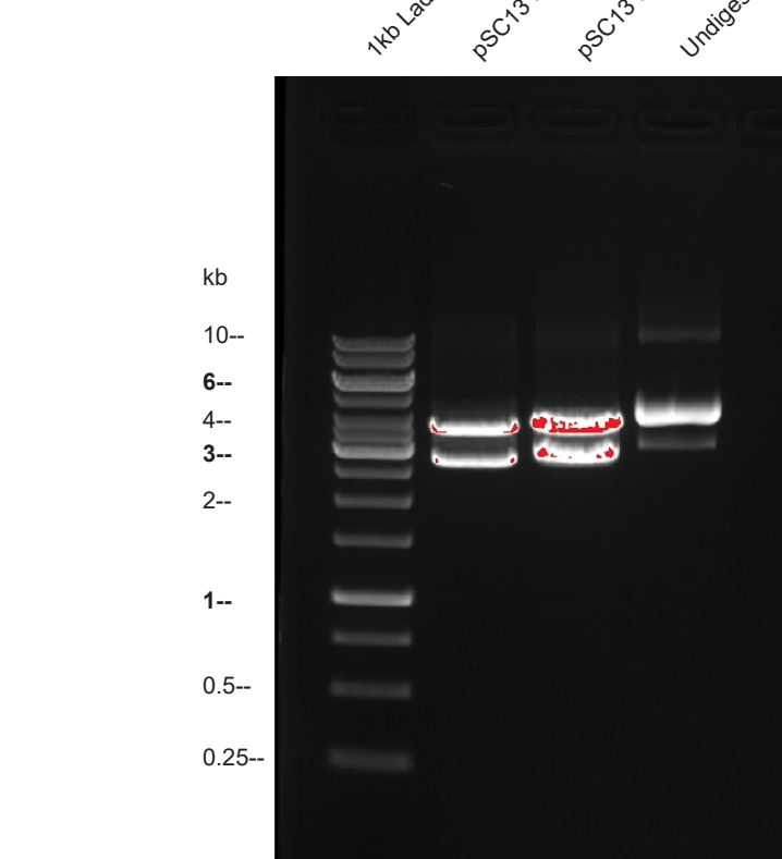
Figure 5: Restriction digest using EcoRI to screen pSC13 colonies visualized on a gel. -With insert bands at 3.5kb and 2.7kb. -No insert bands at 3.5kb and 1kb.
