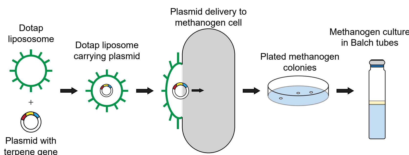
Figure 6: Method of transforming methanogens with terpene plasmids. Successful colonies are streaked for isolation then grown in Balch tubes containing high-salt media with a layer paraffin oil layer.
