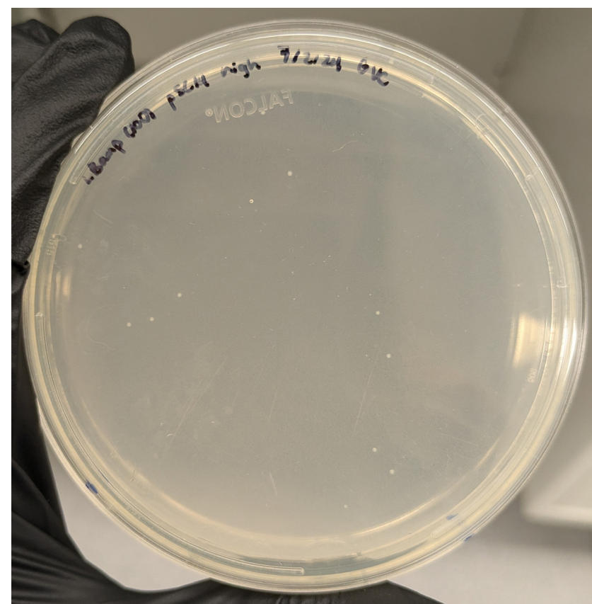
Figure 4: LB ampicillin plate with E. coli colonies containing pSC14.
