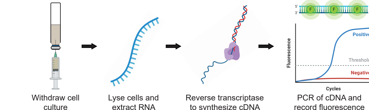
Figure 13: RT-qPCR procedure to check transcription of the terpene genes.
