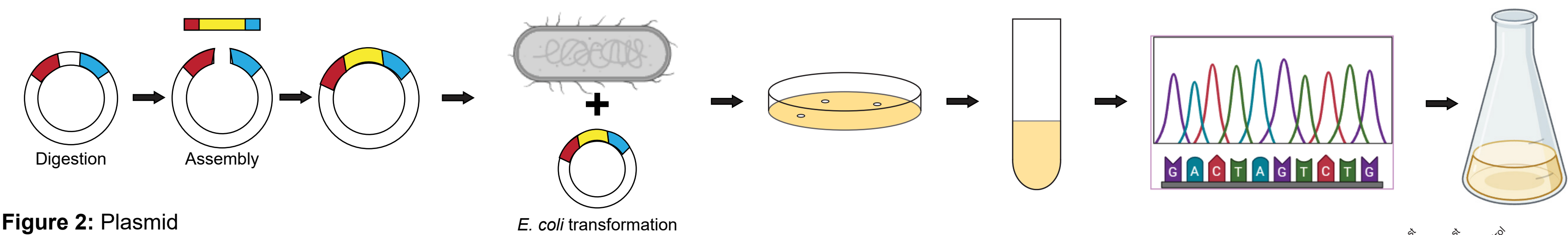
Figure 2: Plasmid assembly using NEB HiFi on digested backbone and terpene gene. Transform plasmid into E. coli via heatshock and plate. Select colonies into LB media with ampicillin. Harvest plasmids, restriction digest screen, and sequence. Correct plasmids are re-transformed and harvested in bulk for methanogen transformations.
