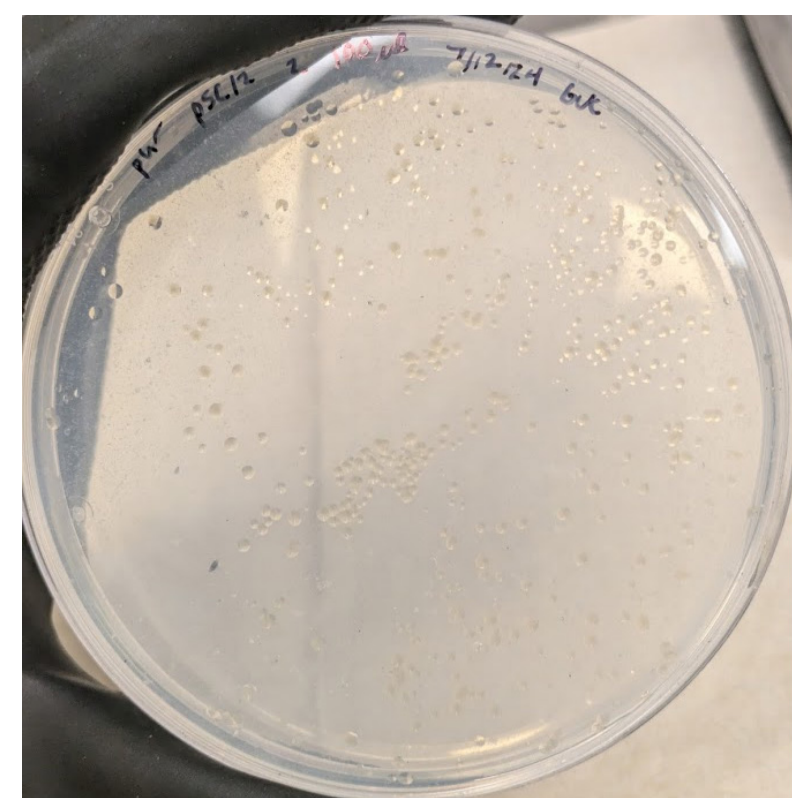
Figure 7: Puromycin selection plate with pSC12 M. acetivorans transformation colonies.
