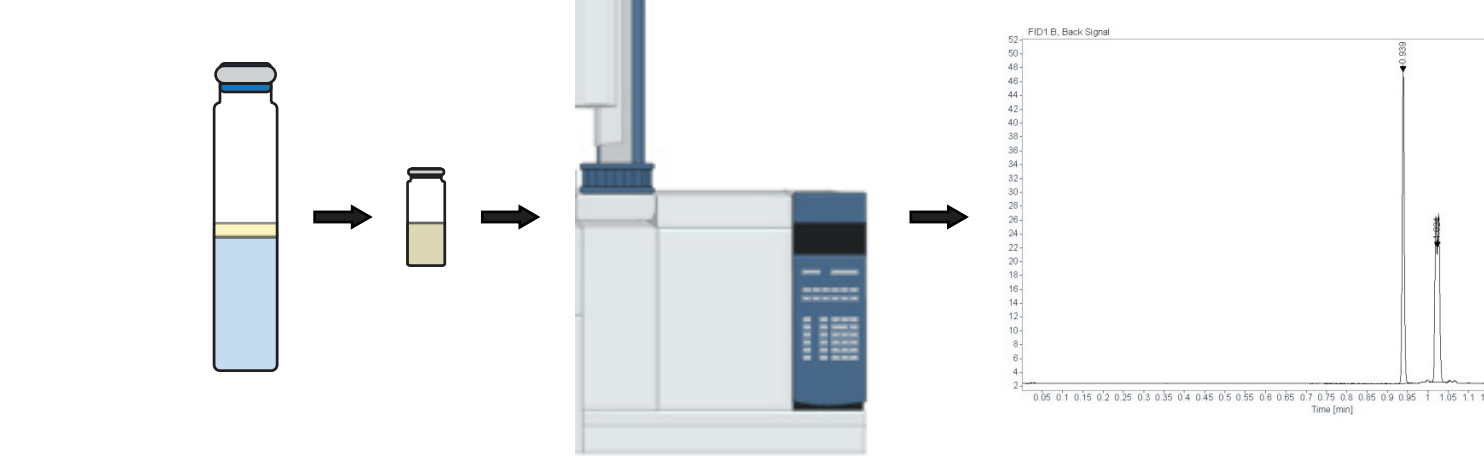
Figure 14: Gas chromatography is performed on the paraffin oil from stationary phase culture. Compare gas chromatogram to the standard terpene in paraffin oil to identify terpene quantities made by methanogens.
