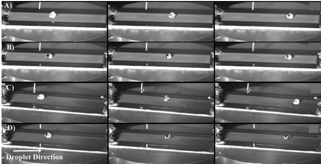
Fig. 7. Droplets at various positions along the leveled sample at temperatures above and below the respective Leidenfrost temperatures. A) 10° sample at 320 °C, B) 10 ° sample at 330 °C, C) 45° sample at 340 °C, D) 45° sample at 360 °C
