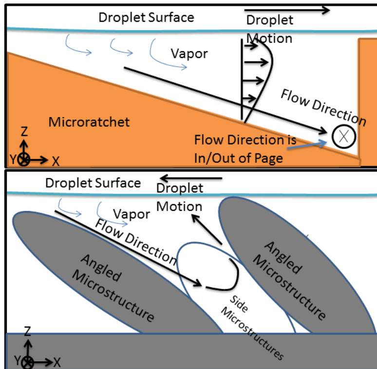
Fig. 8. Top: Schematic describing mechanism governing droplet motion on conventional ratchet microstructures. Bottom: Schematic describing proposed mechanism governing droplet motion on angled FLSP microstructures.
