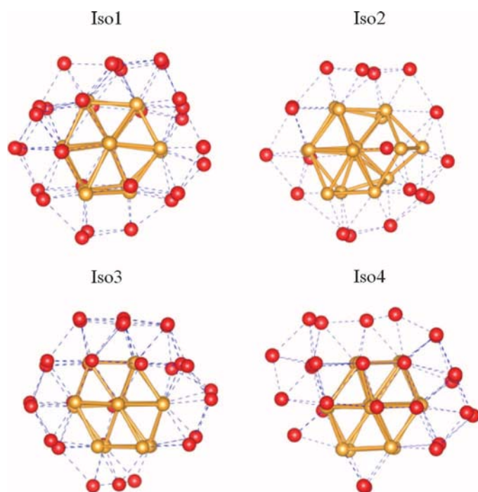
Fig. 3. The fcc-like frameworks of Au 68 in Iso1 to Iso4. The 15 Au atoms in the core are in gold, and the other Au atoms are in red.
