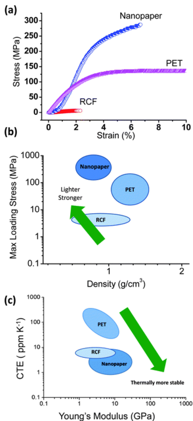
Fig. 3 Mechanical and thermal stability comparison of nanopaper, RCF, and PET. (a) Stress–strain curves of nanopaper, RCF, and PET. (a) Stress–strain curves of nanopaper, RCF, and PET. The nanopaper has the strongest tensile strength. Note that the maximum strain for PET is up to 81%. Ashby plots of (b) maximum loading stress vs. density, and (c) coefficient of thermal expansions vs. Young's modulus.
