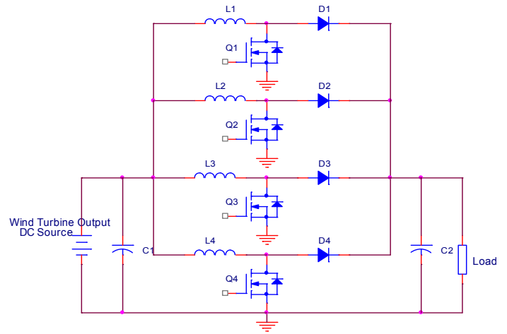
Fig. 3. Schematic diagram of 4-phase interleaved boost converter.
