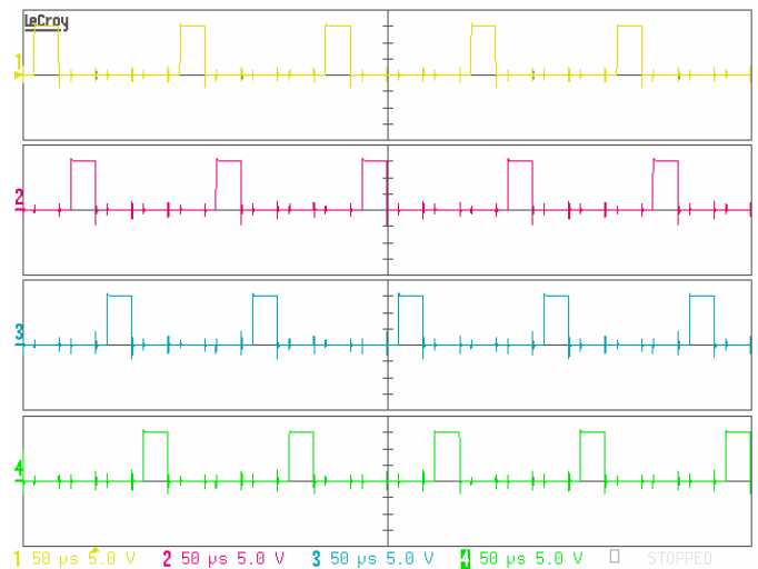
Fig. 9. Gate drive signal waveforms of 4 phases.
