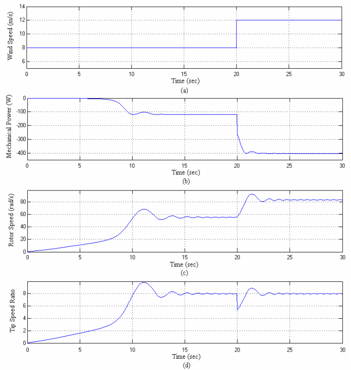
Fig. 6. (a) Wind speed. (b) Mechanical power from turbine (c) Rotor rotational Speed. (d) Tip Speed Ratio.
