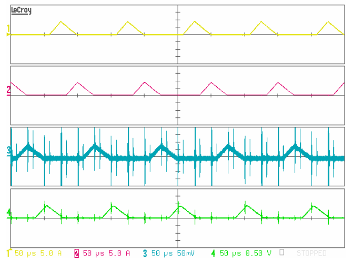
Fig. 10. Inductor current in each phase. (The last two current waveforms have more noise due to different measuring equipment)
