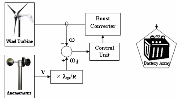
Fig. 1. The block diagram of a wind turbine control system.
