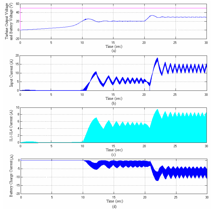
Fig. 7. (a) Wind turbine output voltage vs battery charging voltage (~50V). (b) Input current (sum of 4-phase inductor current) (c) Inductor currents in 4-phases. (d) Battery charging current.
