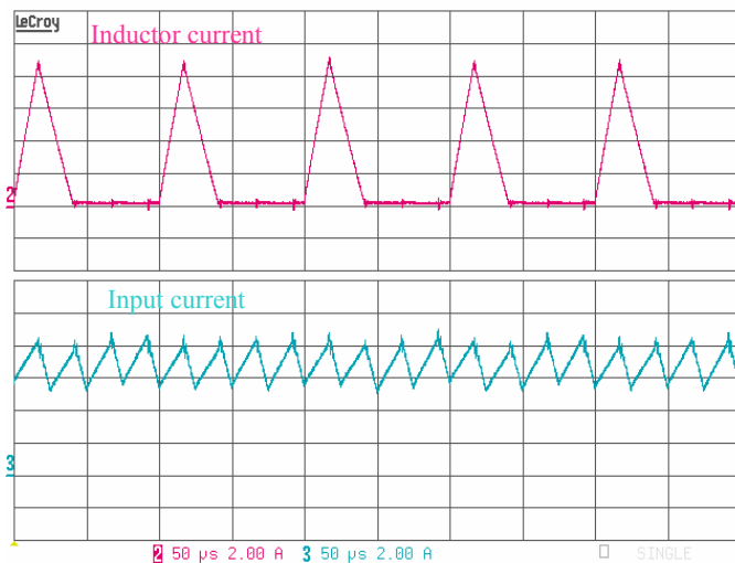
Fig. 11. One phase inductor current vs input current.
