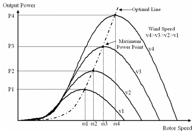
Fig. 2. Output power versus rotor speed at various wind speeds.
