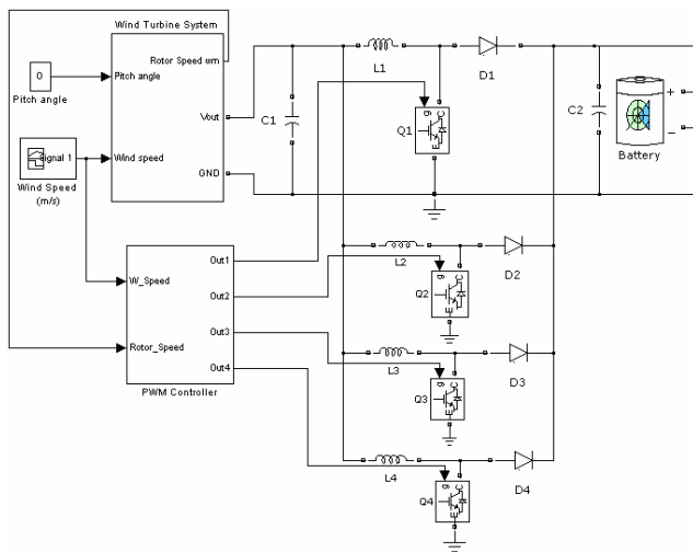
Fig. 5. The model of maximum power extraction from wind turbine system.
